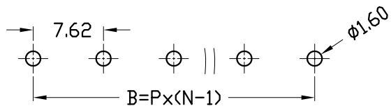
PCB PALOUT
